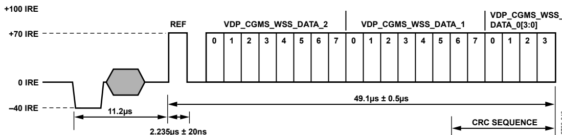
Figure 44. CGMS Waveform
